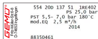
Actuator product label, example: GEMÜ 554
