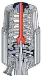
Actuator control function 1 Normally closed (NC)
