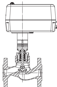
DN 25 to 50
